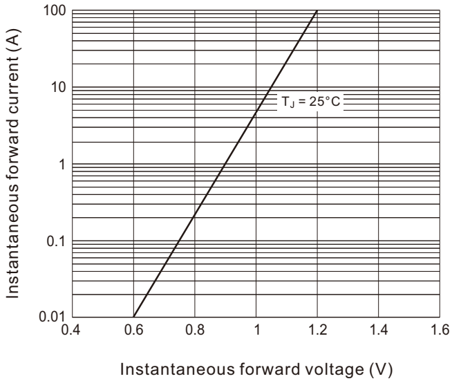
Fig.5 Maximum instantaneous forward characteristics per leg
