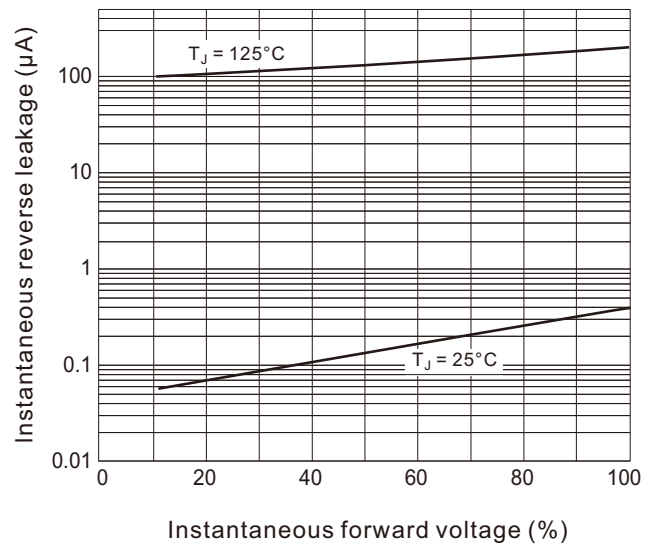
Fig.6 Typical reverse leakage characteristics per leg
