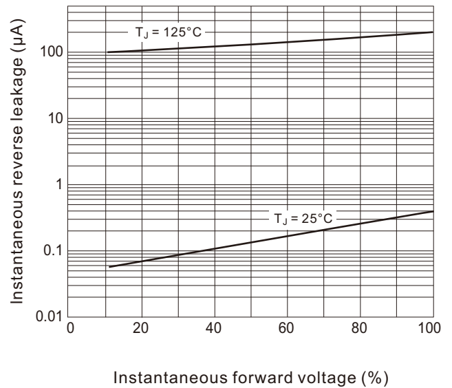
Fig.6 Typical reverse leakage characteristics per leg
