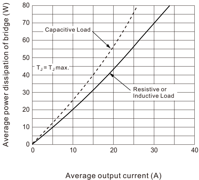
Fig.3 Maximum power dissipation
