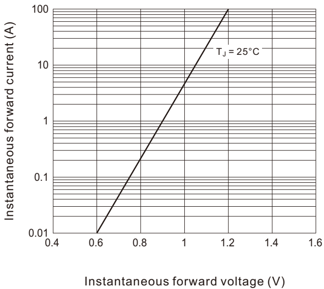
Fig.5 Maximum instantaneous forward characteristics per leg
