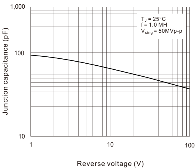
Fig.7 Typical junction characteristics per leg
