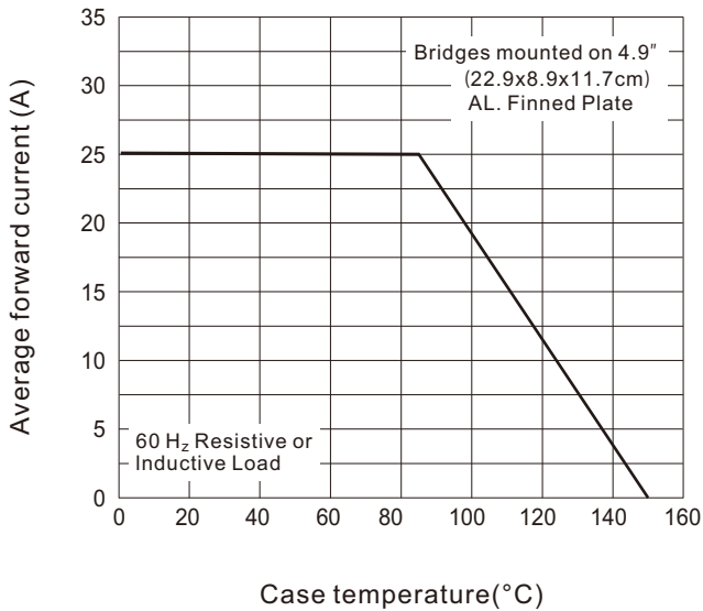
Fig.1 Maximum output rectified current
