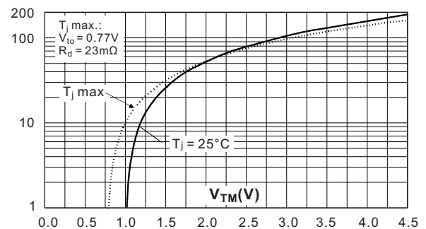
Fig.8 On-state characteristics (maximum values)
